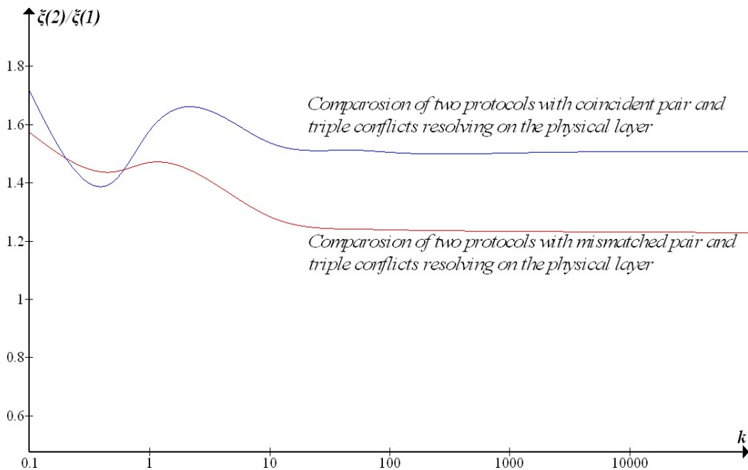
Figure. 5. Comparison of changes in throughput when solving conflicts of multiplicity 2 and 3 under the same conditions of the service.
