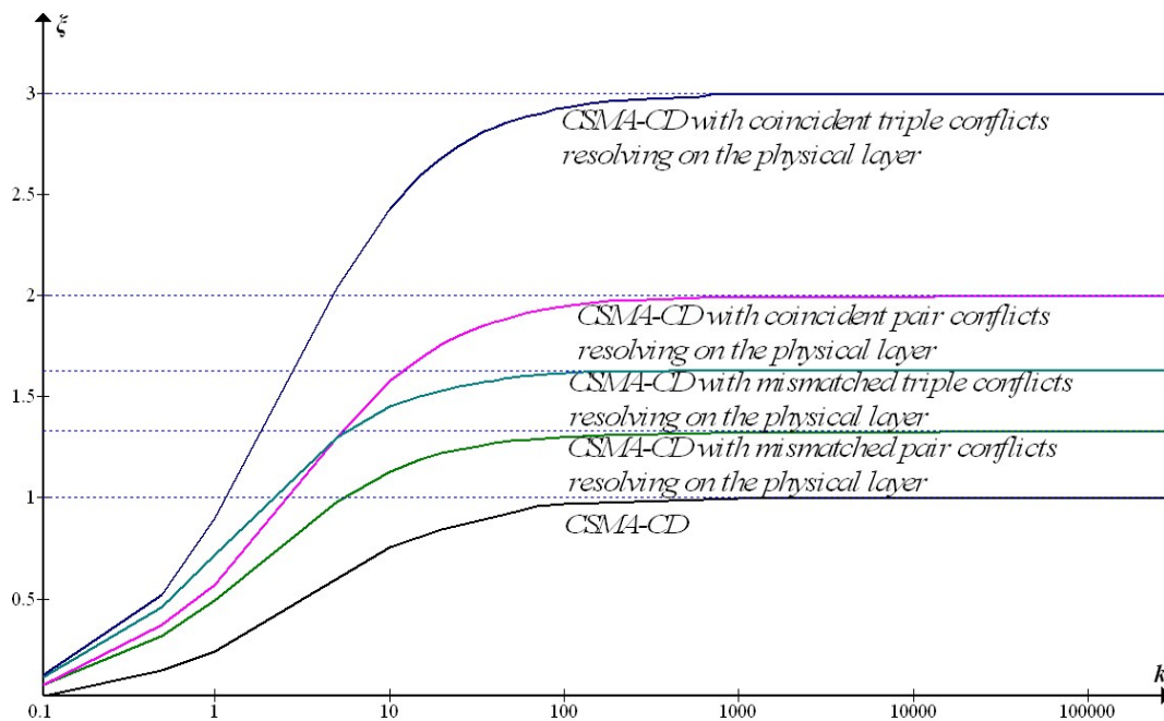
Figure. 2. Throughputs of the CSMA-CD protocols.
