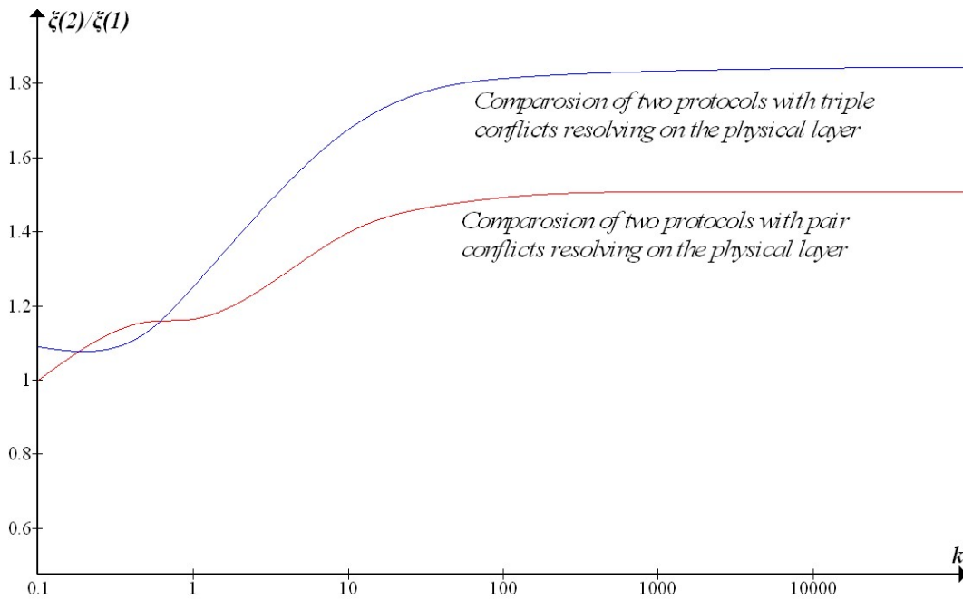
Figure.4. Comparison of CSMA-CD protocols of the same multiplicity by throughput.
