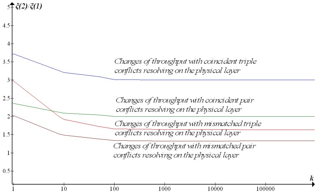
Figure.3. Dependence of relative changes in throughput of CSMA-CD protocols with CRPL with multiplicity 2 and 3 on the relative intensities of service on 1 and 2 stages.
